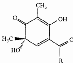
13 R = \text{C}_3\text{H}_7
